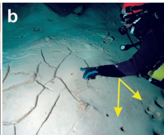
Figure 41: a) Desiccation polygons in the Sector de les Grans Sales. b) Desiccation polygons and dripping impact marks in the Collonuda Nord gallery (Sector Subaquàtic de Gregal). (Photos M.A. Perelló and J. Pocoví).
